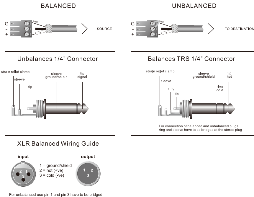
[ Figure 2.1 Input wire and connectors ]
