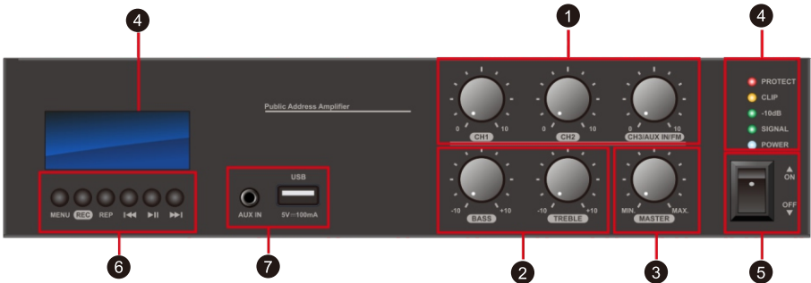
[ Figure 1.1 Front panel diagram ]
